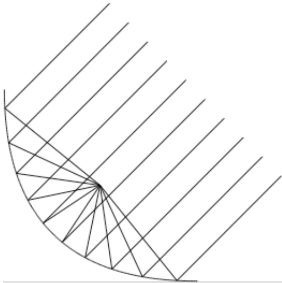
“classic” design (parabola)
